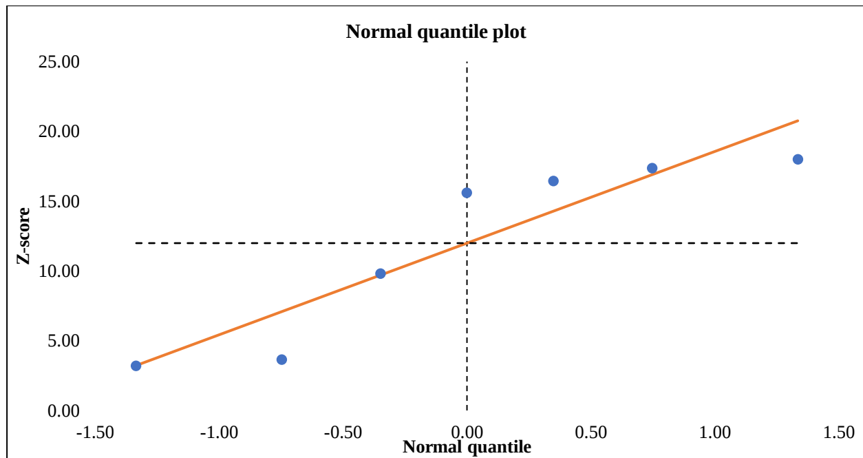
Figure 6. Normal quantile plot
