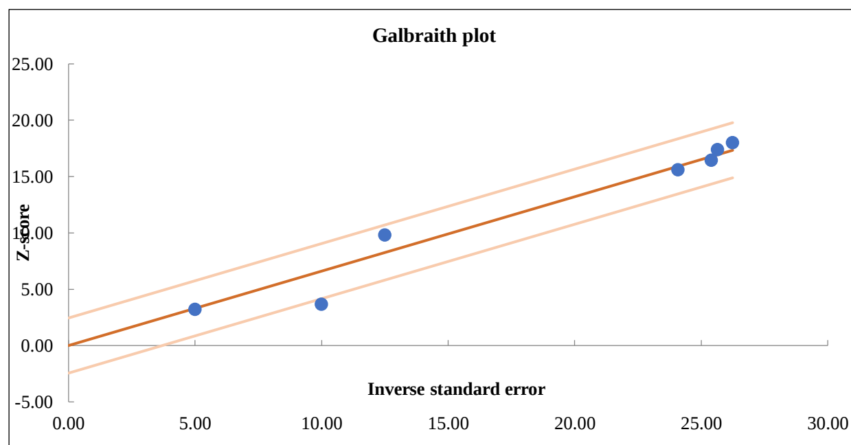
Figure 5. Galbraith plot
