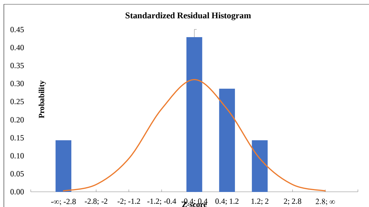
Figure 4. Standardized residual
