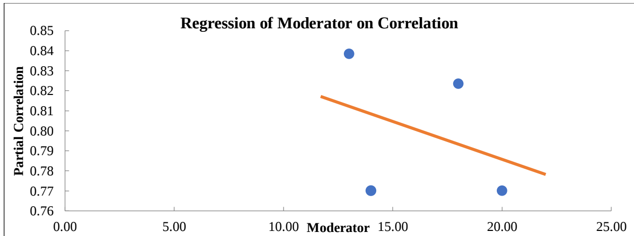
Figure 2. Regression of moderator on the correlation
