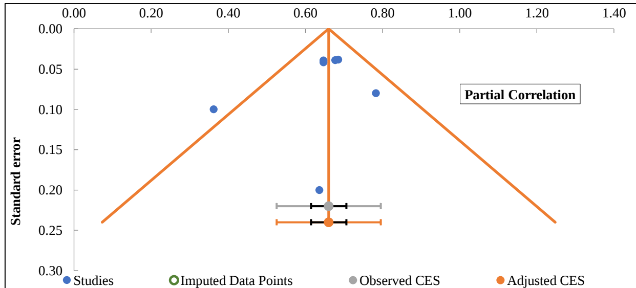
Figure 3. Funnel plot
