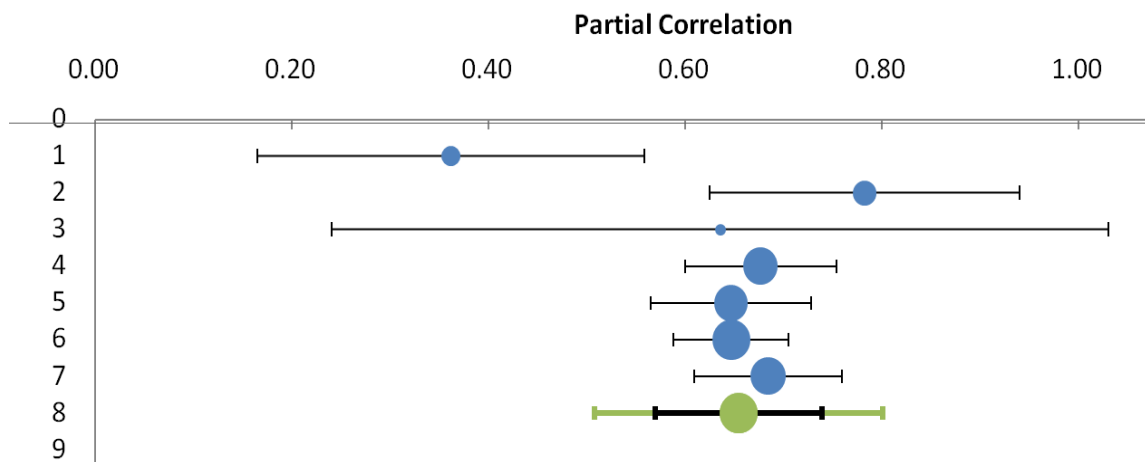
Figure 1. Forest plot
